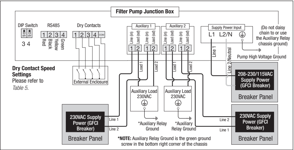
Figure 12. 208-230V Auxiliary Relay Wiring Diagram*
