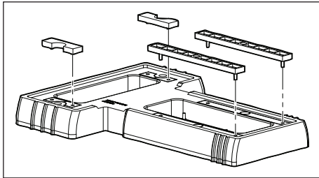
Figure 7. Snap Spacers Into Place
