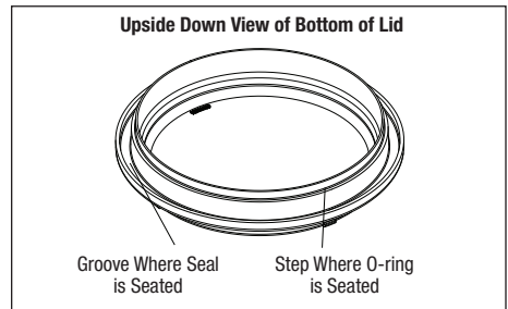
Figure 16. Placement of Blue Pressure Test O-ring
