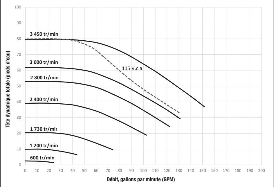
Courbes de performance VSSHP220DV2A(S)
