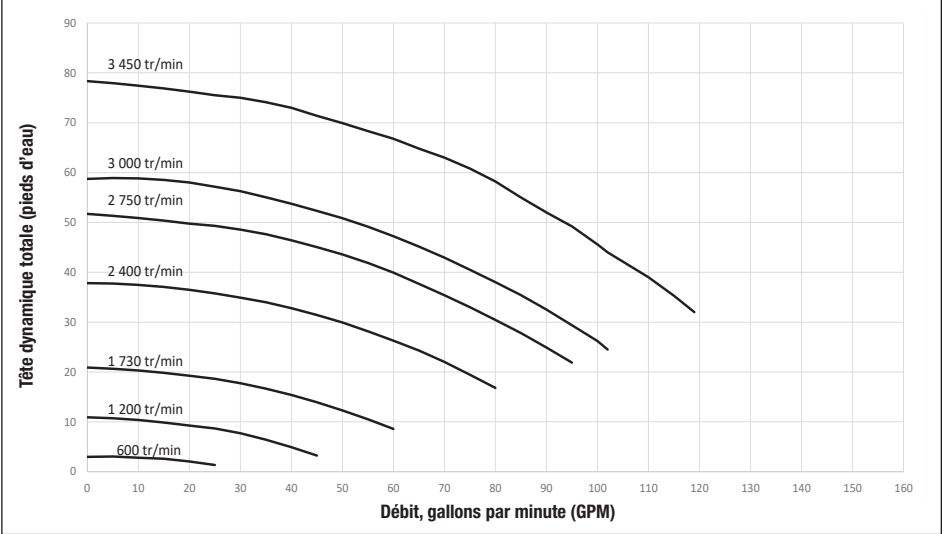
Courbes de performance VSFHP185DV2A(S)
