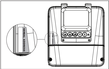
Figure 10. Serial Address Label Location
