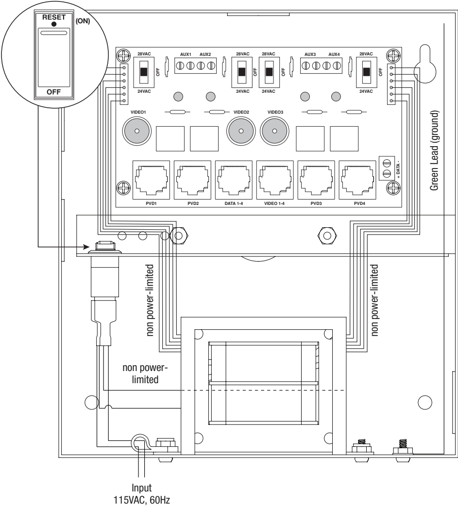
Fig. 4a - Illuminated master power disconnect circuit breaker: • OFF position: circuit breaker tripped – Switch not illuminated. • RESET (ON) position – Switch illuminated.
