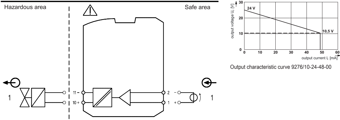
9276/10-21-25-00 connection diagram
