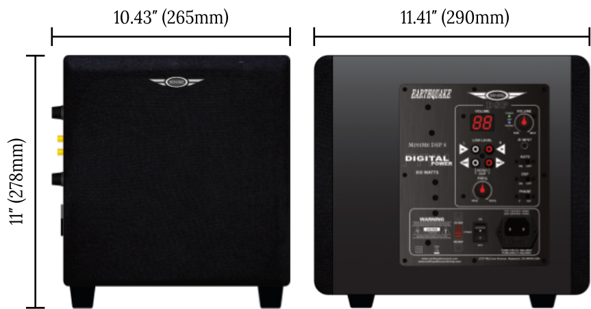
DIMENSIONS INCLUDE FEET, GRILLE, AND AMPLIFIER
