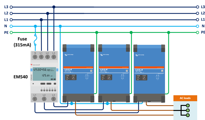
EM540 wired as a 3-phase Grid meter
