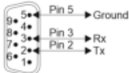
Figure 4: RS-232 Pinout
