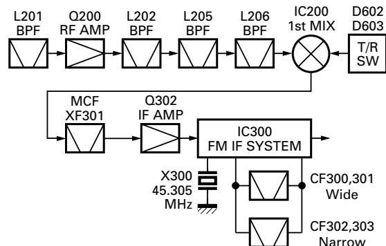
Fig. 2 Receiver section
