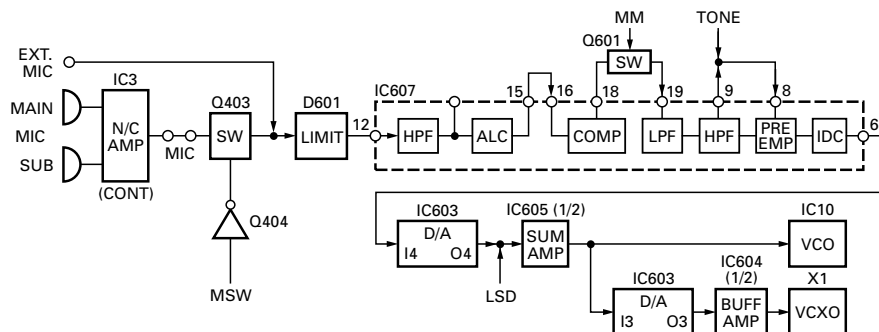
Fig. 6 Microphone circuit
