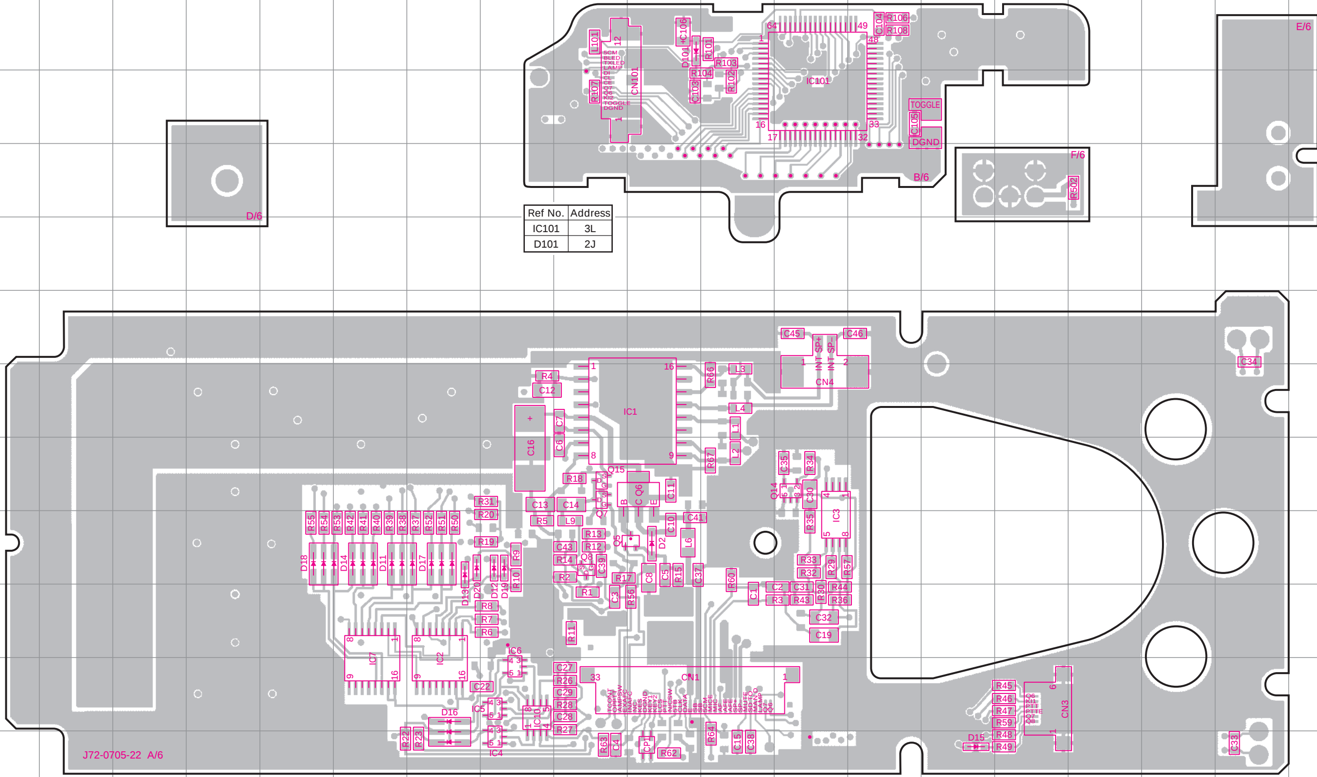
CONTROL UNIT (X53-3930-XX) -11 : K -12 : K2 Foil side view
