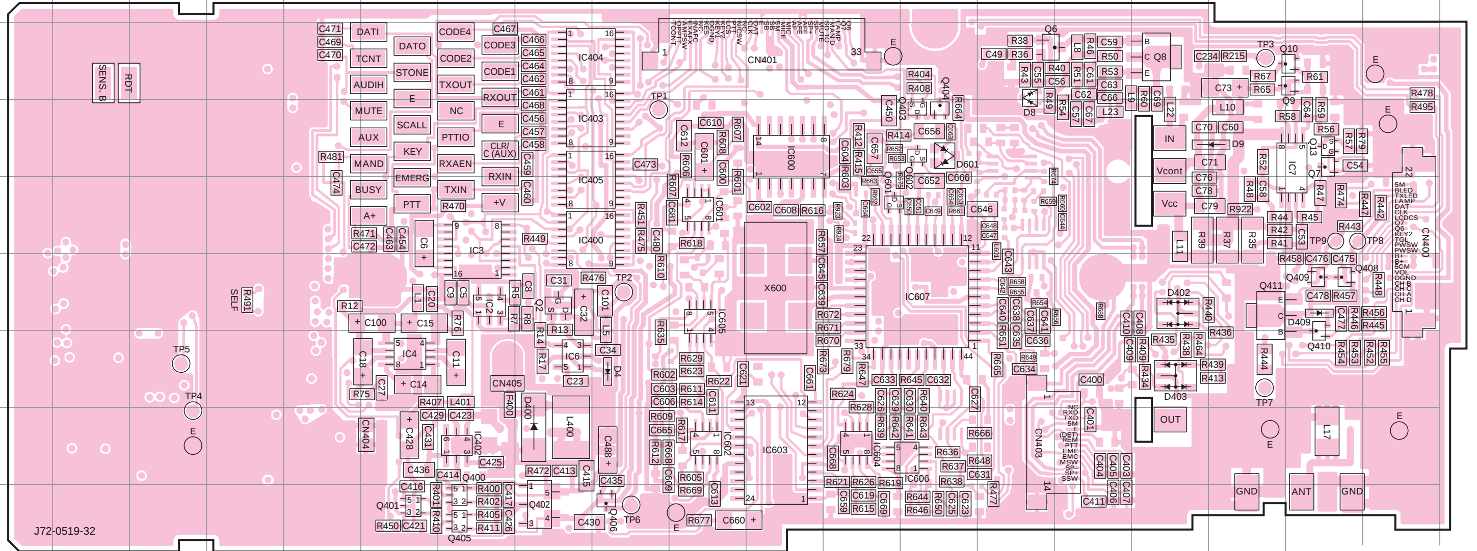
TX-RX UNIT (X57-5390-10) Component side view
