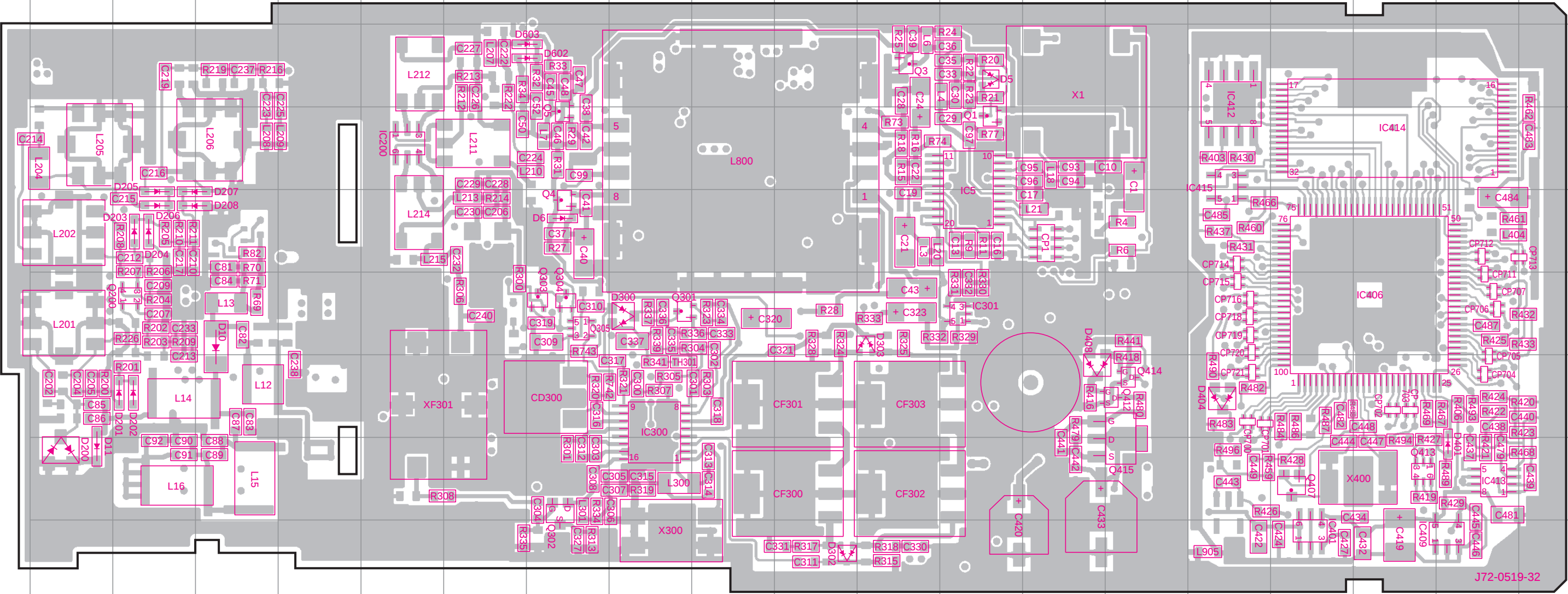
TX-RX UNIT (X57-5390-10) Foil side view
