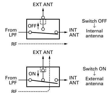
Fig. 8 Internal-External antenna switching
