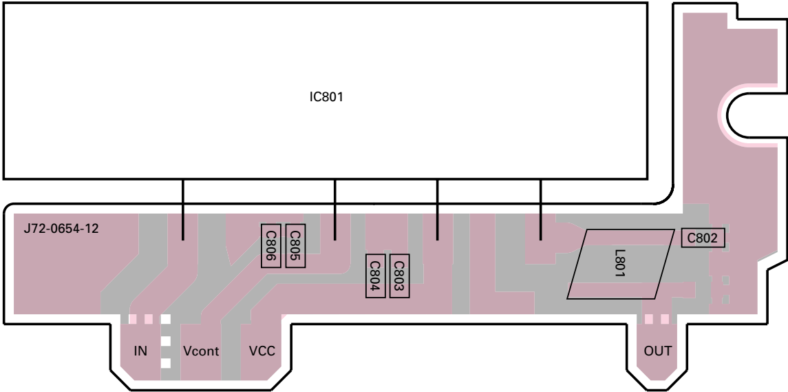
FINAL UNIT (X45-3592-71) Component side view
