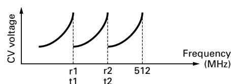
Fig. 10 CV voltage vs frequency
