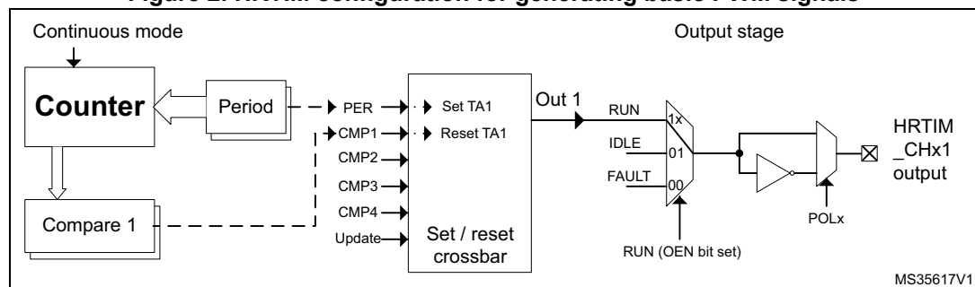
Figure 2. HRTIM configuration for generating basic PWM signals
