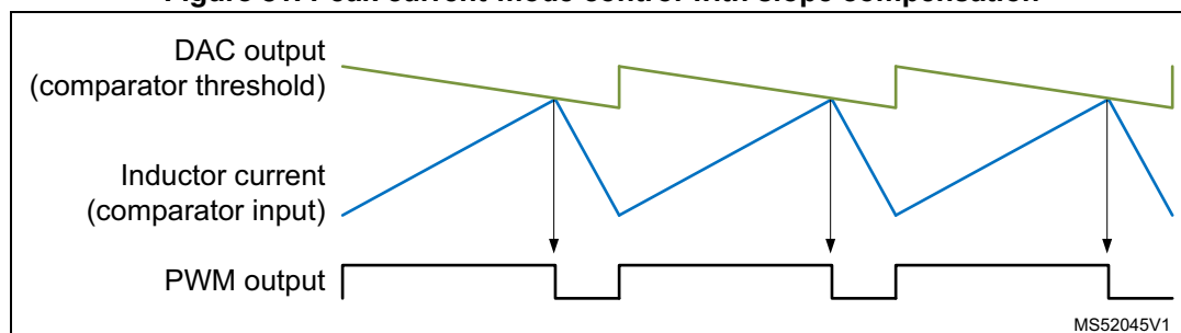
Figure 31. Peak current-mode control with slope compensation
