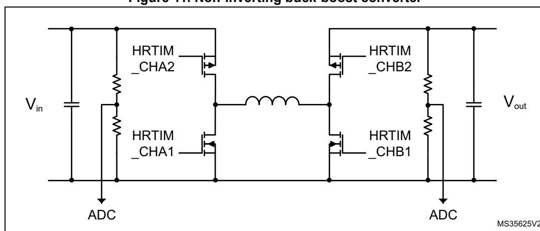
Figure 11. Non-inverting buck-boost converter
