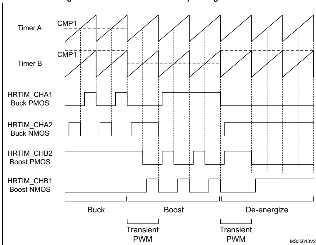
Figure 13. Buck-boost converter operating waveforms
