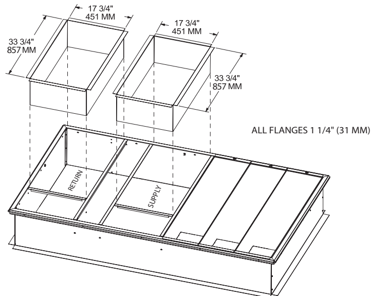
Figure 19. Cooling with Optional Electric Heat and Gas/Electric Models 6-10 Tons - Downflow Duct Connections Field Fabricated
