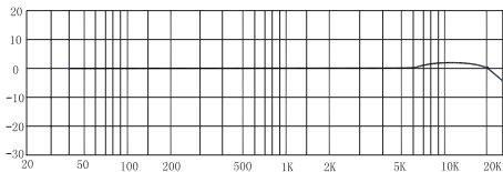
Frequency Response
