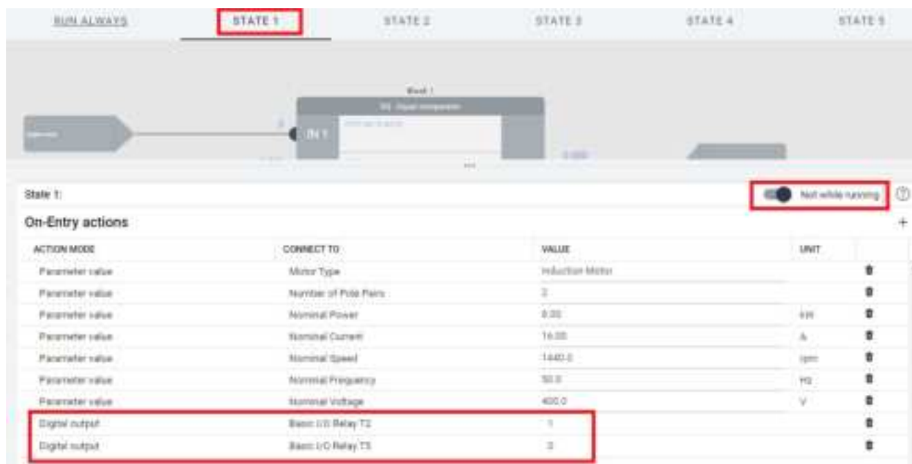
Illustration 19 : Example: Multi motor, State 1, Induction motor
