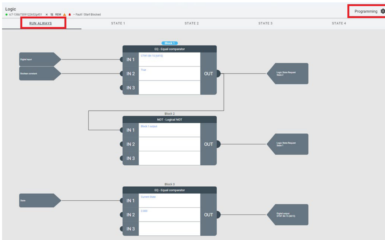
Illustration 18 : Example: Multi motor, State selection in Run Always-Tab
