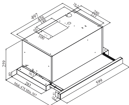
Figure 2 – Range hood dimensions
