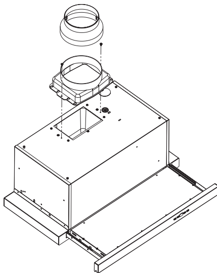
Figure 4 - Installation of non-return flap and adapter
