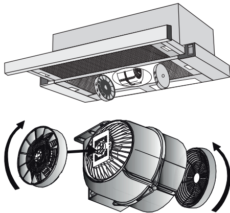
Figure 10 - Installation of charcoal filters
