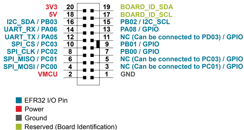
Figure 3.5. EXP Header
