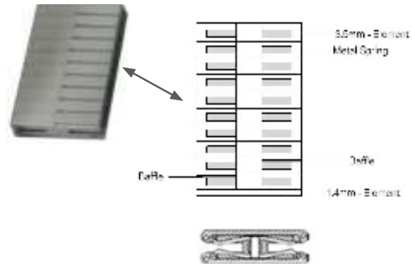
Figure 6: Board-to-Board Connector
