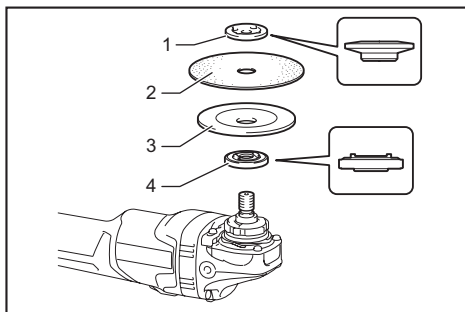
► 1. Sanding lock nut 2. Abrasive disc 3. Rubber pad 4. Inner flange
