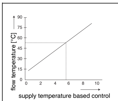
Fig. 1 0 - 10V Diagram
