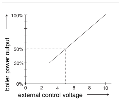
Fig. 2 Control based on power output
