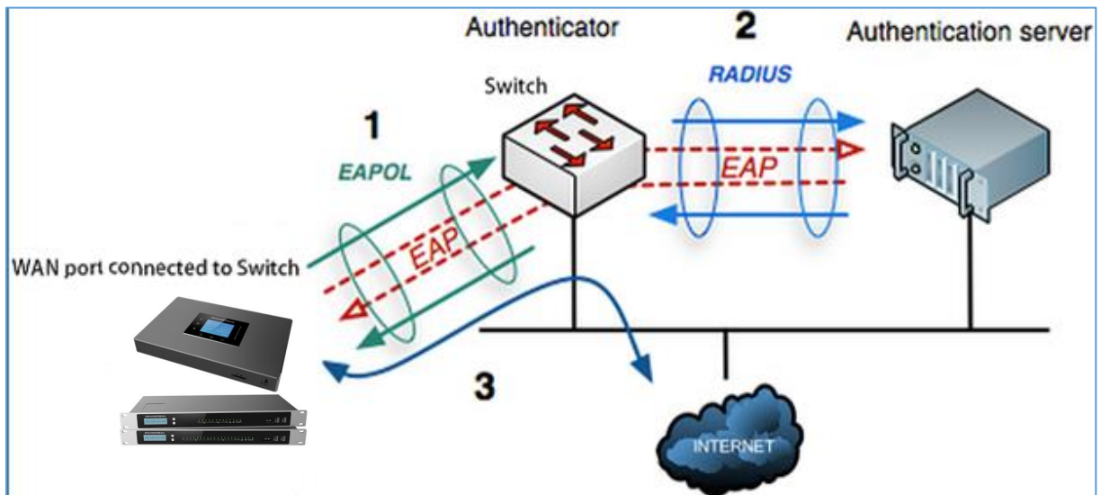
Figure 19: UCM630X Using 802.1X as Client
