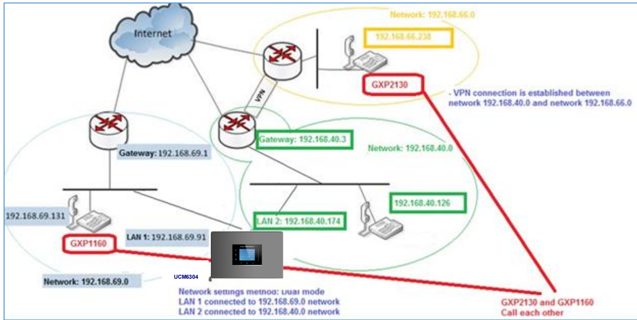
Figure 21: UCM6304 Static Route Sample
