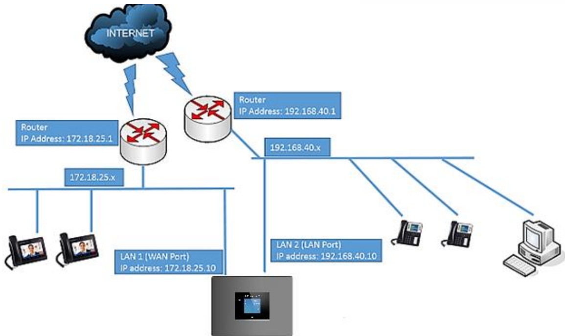
Figure 18: UCM6302 Network Interface Method: Dual
