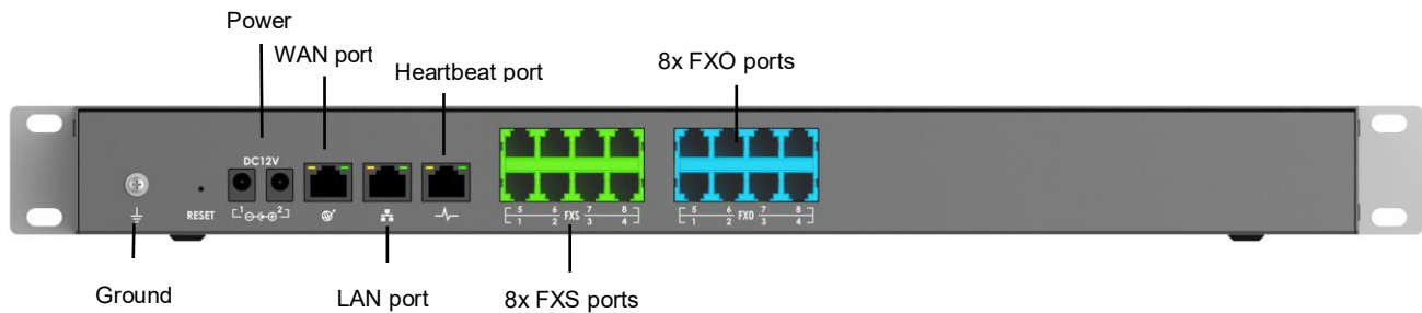
Figure 9: UCM6308 Back View
