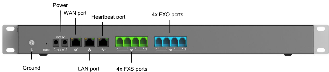
Figure 6: UCM6304 Front View
