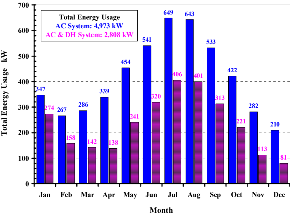
Figure 4. Total Energy Usage vs. Month for Strategy 2
