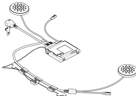
e-box with wiring
