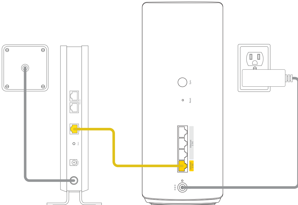
Figure 3. Connect the router to a modem
