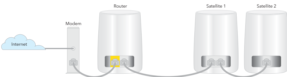
Figure 5. Daisy chain topology: Satellite 1 connected to router and satellite 2 connected to satellite 1
