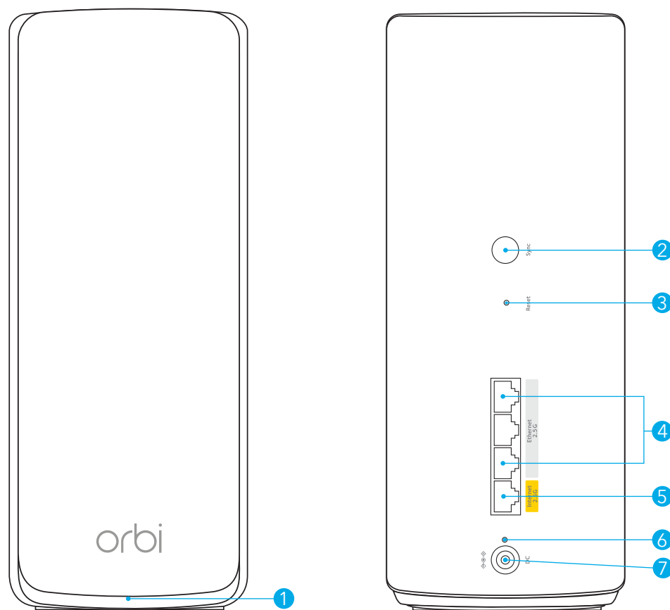
Figure 1. Orbi router front (left figure) and back (right figure) views
