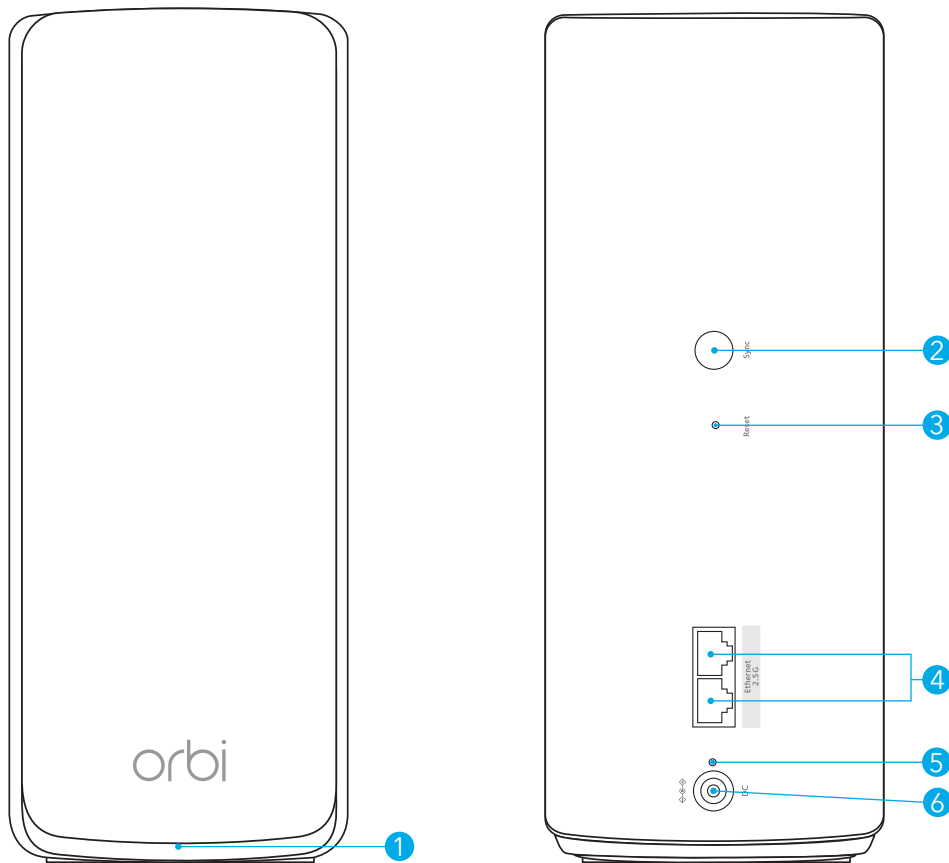
Figure 2. Orbi satellite front (left figure) and back (righth figure) views
