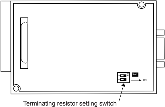
Terminating resistor setting switch Rear view of RS-422/485 communication unit.
