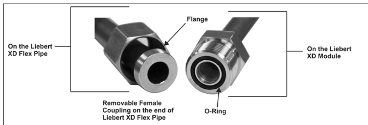
Figure 6.13 Removable couplings
