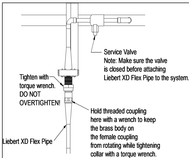
Figure 6.18 Detail view of Liebert XD Flex Pipe and prefabricated piping port
