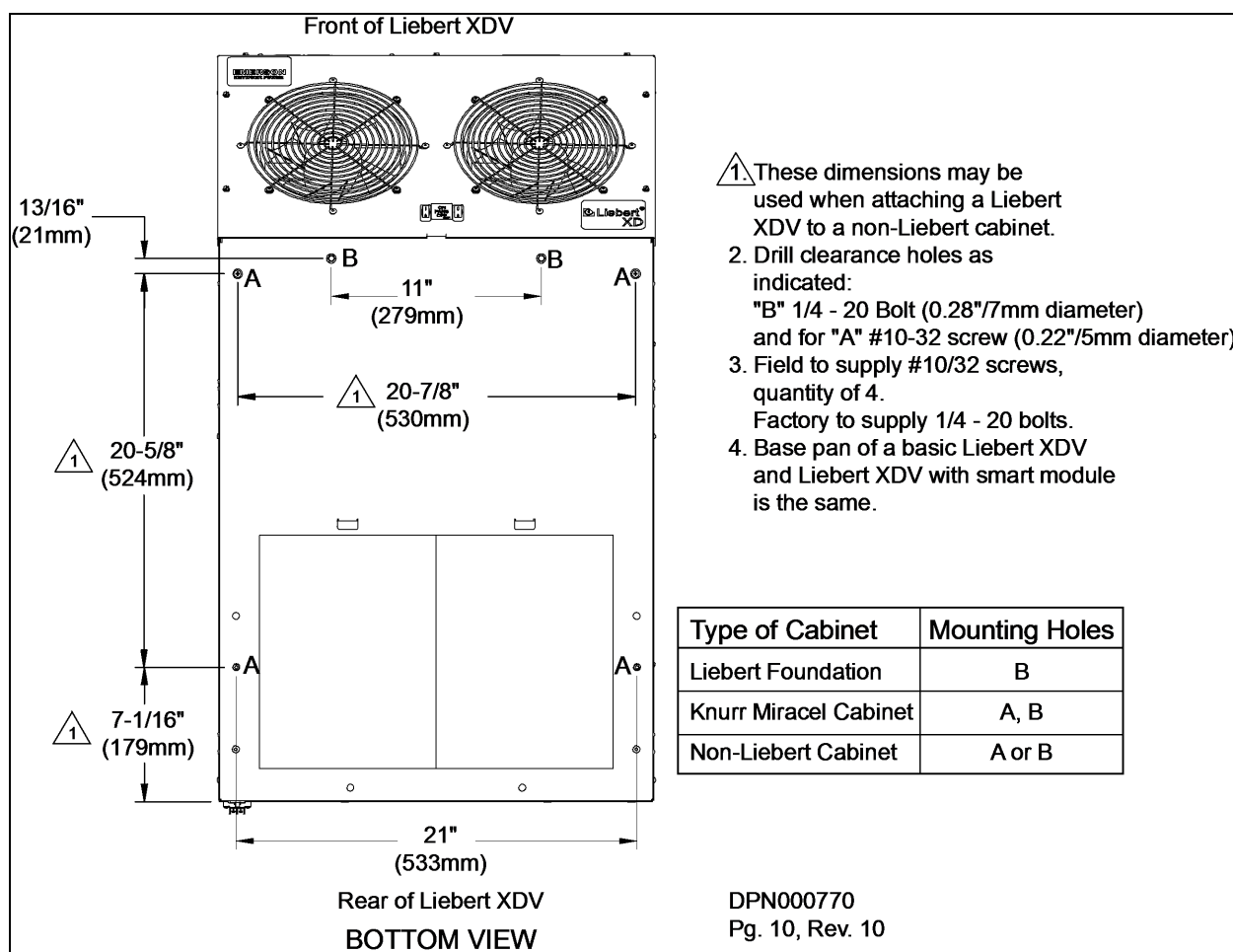
Figure 5.3 Mounting hole locations—alternate mounting points
