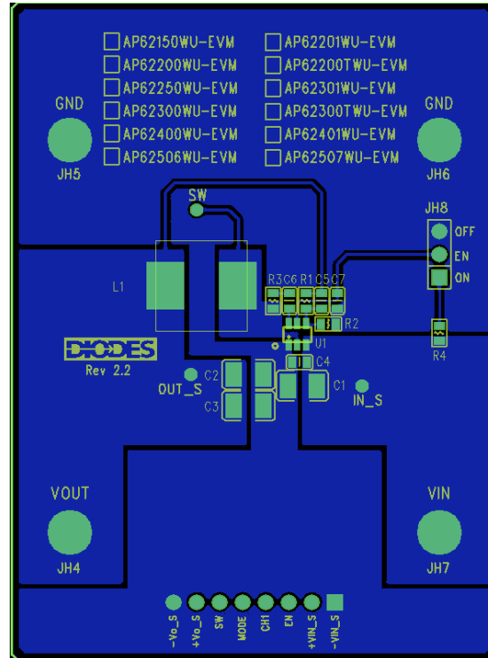
Figure 3. AP62300WU-EVM – Top Layer
