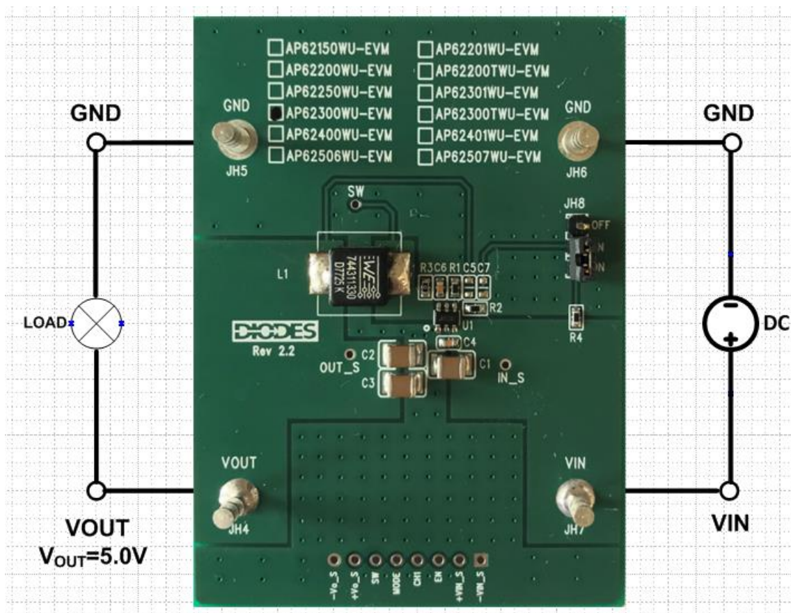
Figure 1. AP62300WU-EVM
