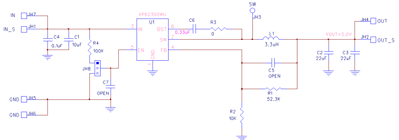
Figure 2. AP62300WU-EVM Schematic
