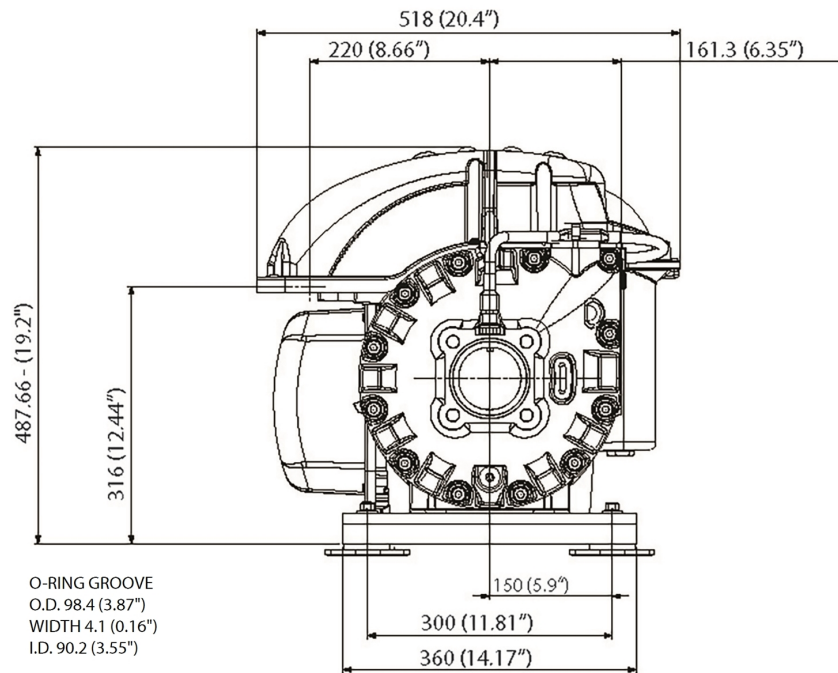
Figure 16-2 Service Side View (Excluding TTH/TGH Compressors)
