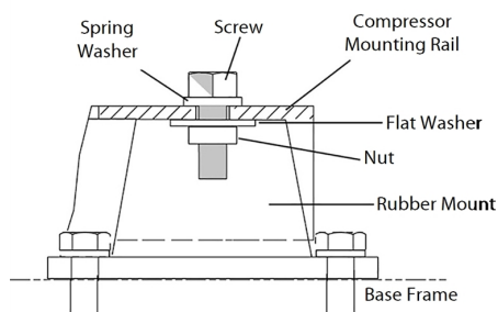
Figure 20-4 Correct Compressor Mounting Pad Installation
