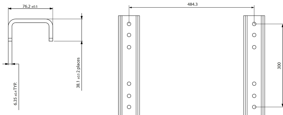
Figure 20-2 Mounting Base (TTS/TGS/TTH/TGH) Series
