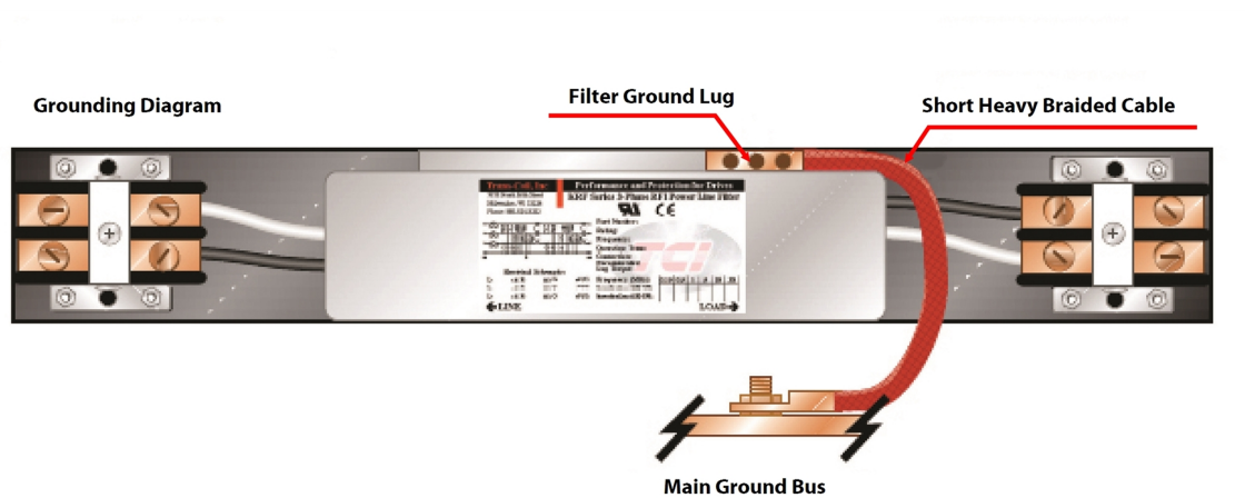
Figure B-2 Grounding Diagram
