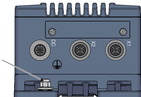
Figure 8. Earth connection
