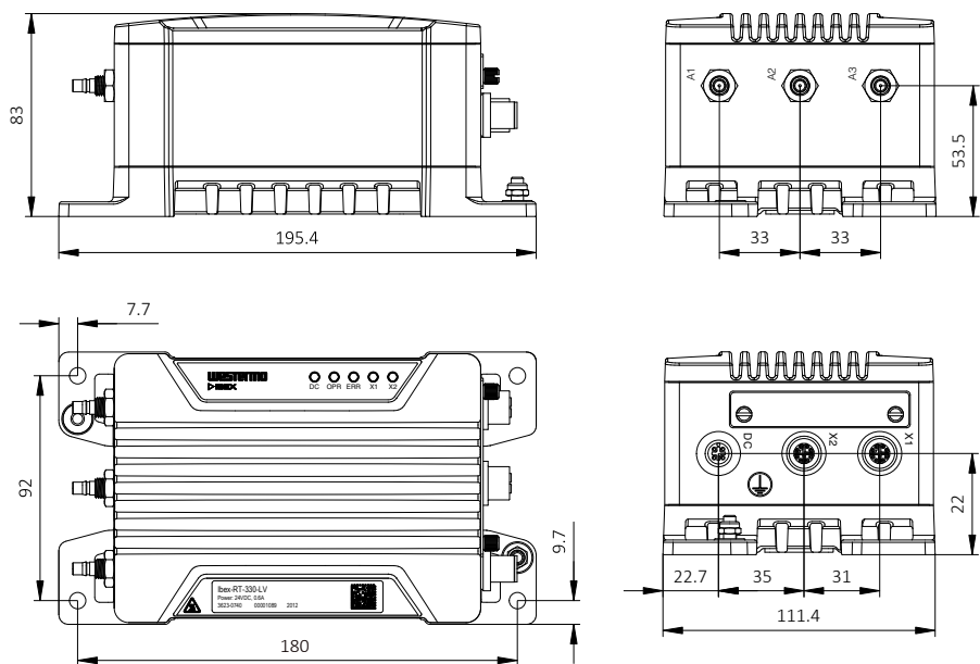
Figure 7. Dimensional drawing
