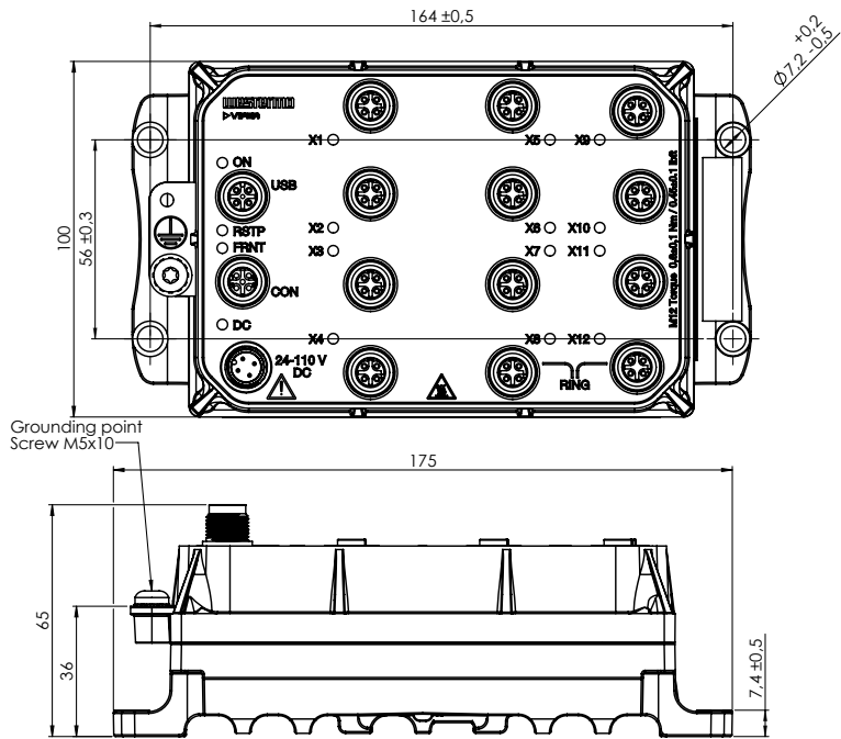
Figure 4. Dimensional drawing
