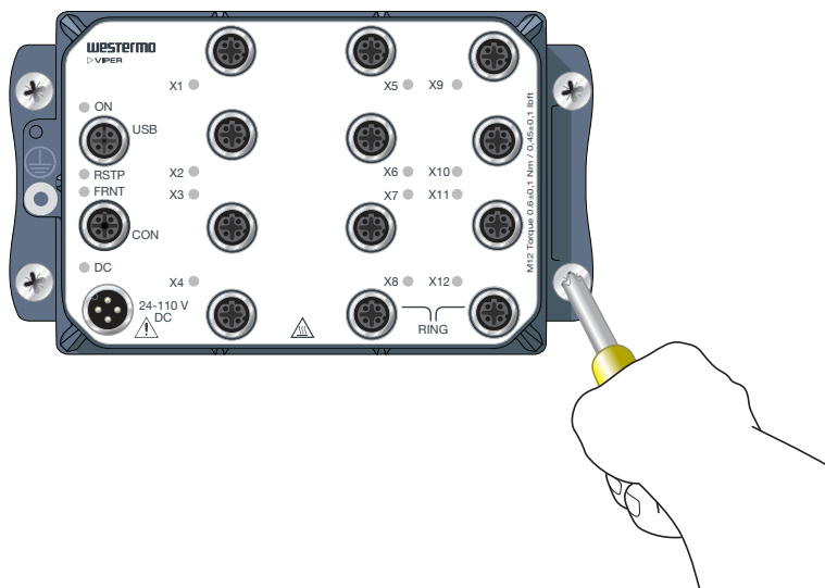
Figure 5. Wall mounting
