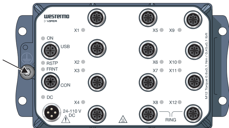
Figure 6. Earth connection
