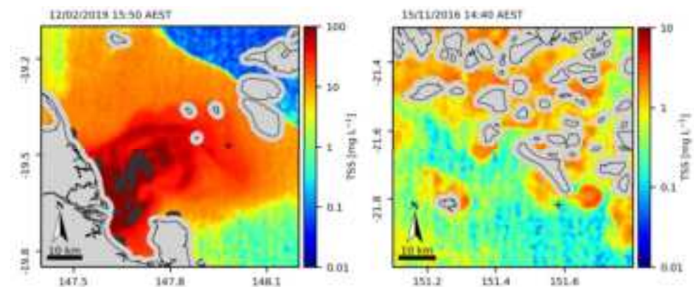
Figure 7. Flood plume discharging from the Burdekin River, February 2019 (left panel). TSS tidal jets within the GBR reef matrix in November 2016 (right panel). Note the different ranges in each plot. Pixels masked in black are due to out-of-range TSS values.
