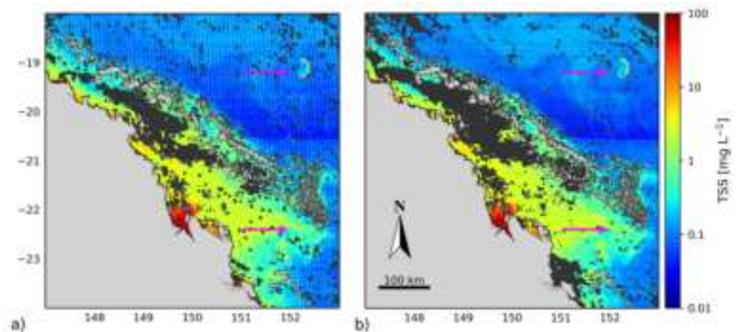
Figure 12. Location of transects (magenta arrows) extracted for \text{TSS}_{\text{SING}} (a) and \text{TSS}_{\text{AGG}} (b). Note the cumulative cloud masking in \text{TSS}_{\text{AGG}} . Himawari-8 observations taken on 9 September 2017 between 10:00 and 10:50 local time (AEST).
