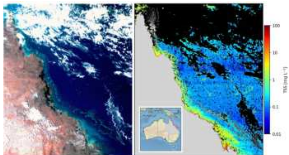
Figure 6. Near-true colour Himawari-8 imagery of the GBR acquired on 27 October 2017 at 15:00 AEST (left panel) and the associated TSS product [ \text{mg L}^{-1} ] (right panel). Pixels masked in black due to clouds and out-of-range values.
