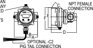
CTx (shown with -C2 pig tail connection)
