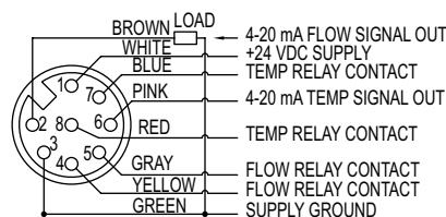
PIN connector standard wiring
