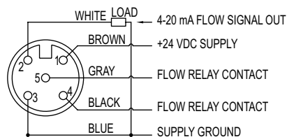
CP [FLOW ONLY] WIRING
