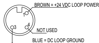
CX2 wire transmitter
