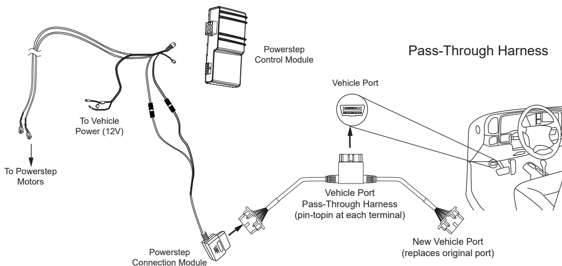
OBD II Module located below steering column.
