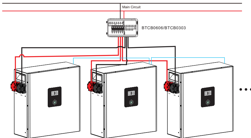
Figure 3-2 Multiple Battery Parallel System Connection Diagram
