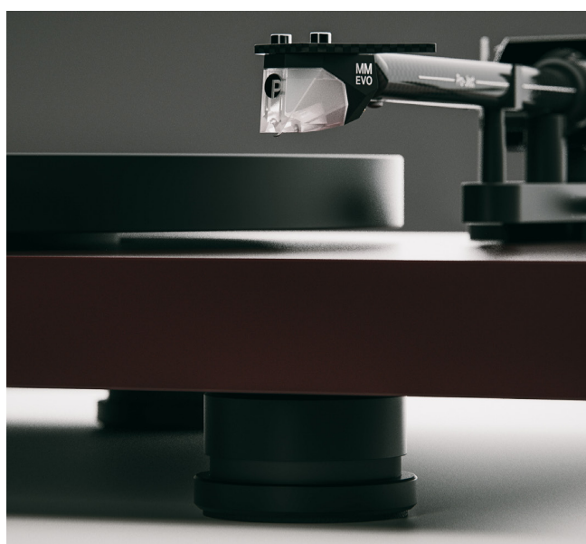
TPE damping part for decoupling
