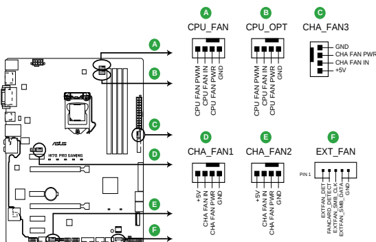
H170 PRO GAMING Fan connectors
