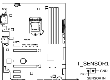
H170 PRO GAMING T_SENSOR connector
