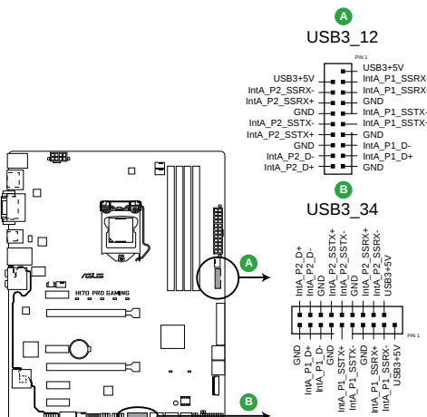
H170 PRO GAMING USB3.0 Front panel connectors
