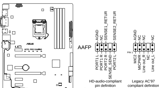
H170 PRO GAMING Front panel audio connector
