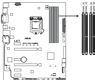
H170 PRO GAMING 288-pin DDR4 DIMM soc
