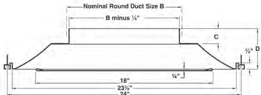
Model: OMNI 3N (for Narrow Tee)
