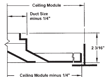
MCD3 (24" x 24" Lay-in)
