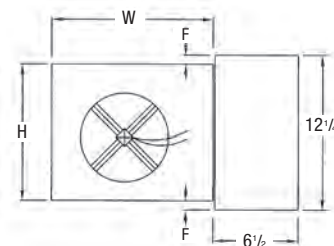
AESV with optional Control Enclosure
