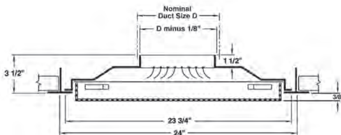
Model: PCS3D (Drop Screen Lay-In)
