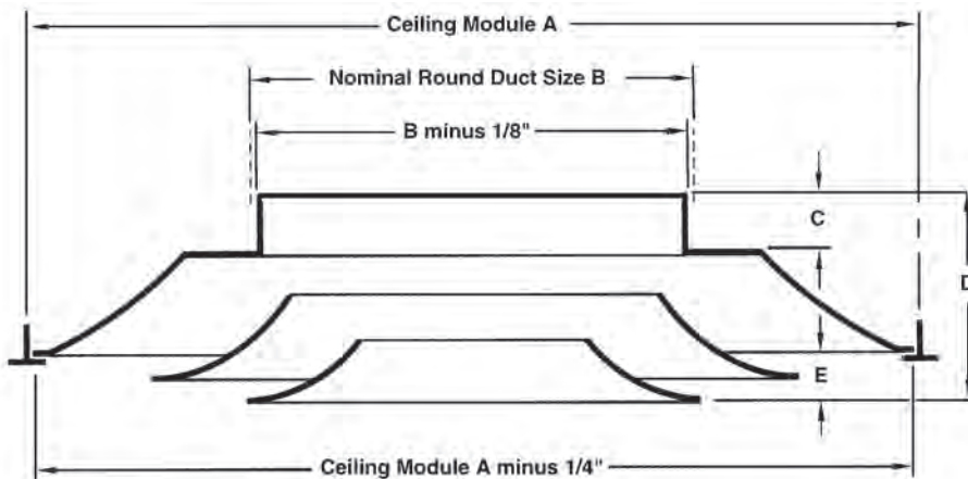
Model: TMS Frame Type 3 (Lay-In)
