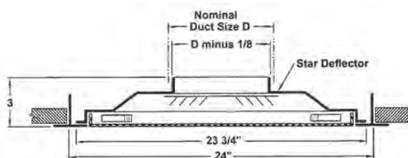
Model: PSS3F (Standard Lay-In)
