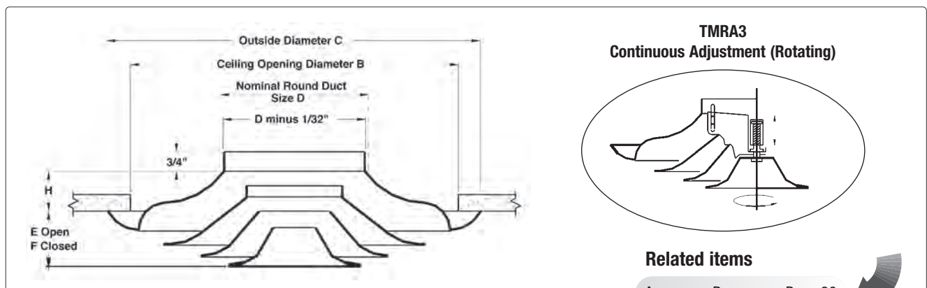
Model: TMRA3 – Horizontal to Vertical Discharge Patterns
