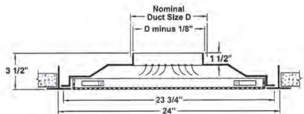
Model: PCS3F (Standard Lay-In)
