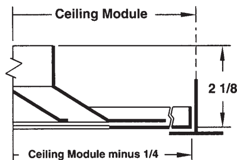
TDC3 (24"x 24" Lay-In)
