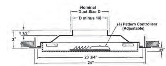
PDS3D (Drop Screen Lay-In)
