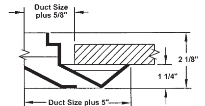
MCD6 (Beveled Surface Mount)
