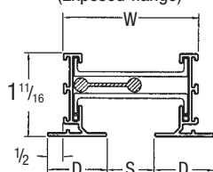
Border Type 66 (1 Slot) (Exposed flange)
