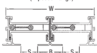
Border Type 66 (2 Slot 2CRA) (Exposed flange)
