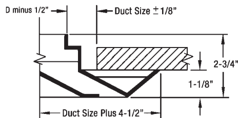
TM6 (Surface Mount, Beveled Frame)
