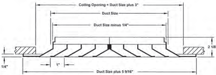
MCD1 (Flush Surface Mount)
