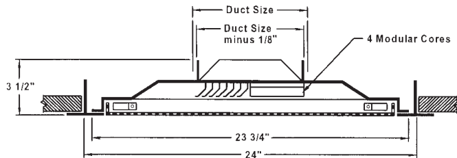
Model: PMC3F (Standard Lay-In)
