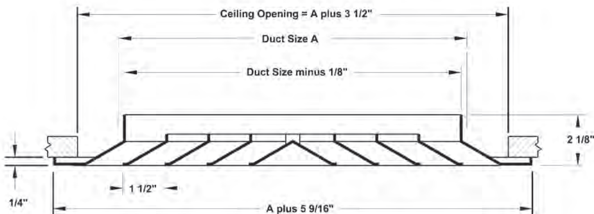
TDC 1 (Surface Mount)
