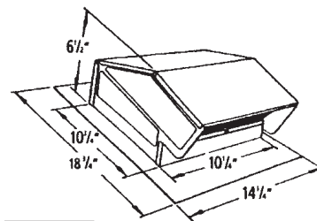
Sloped Roof/Wall Caps Model: 634
