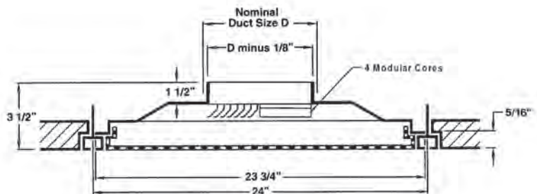
Model: PMC3N (for Narrow-Tee)
