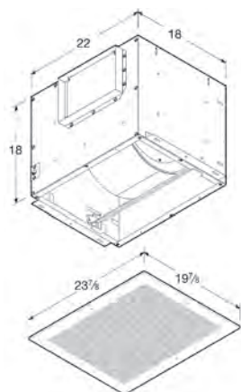
Models T/L900 & T/L1500
