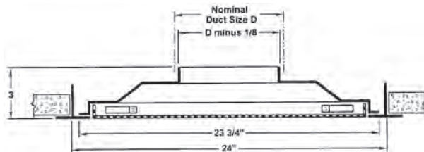
PAR3F (Standard Lay-In)
