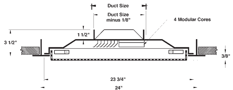
Model: PMC3D (Drop Screen Lay-In)
