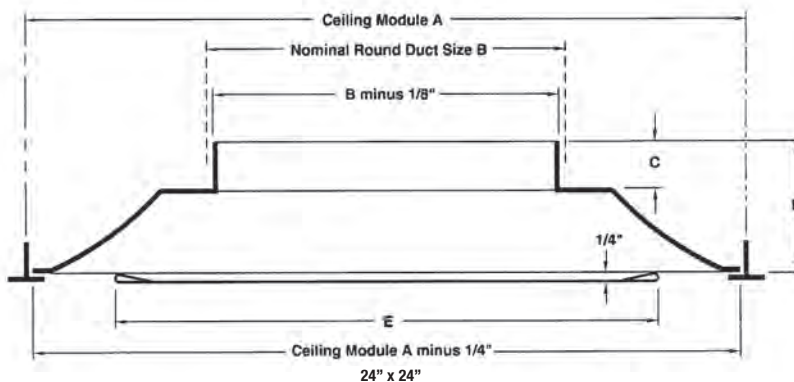
Model: OMNI Frame Type 3 (Lay-In)
