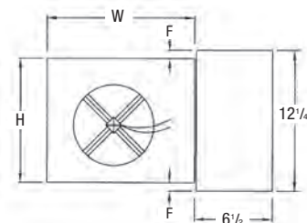
DESV with optional Control Enclosure
