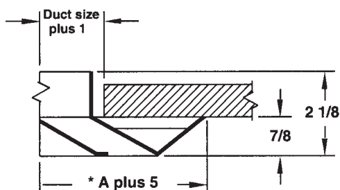
TDC6 (Surface Mount)
