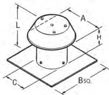
Model: RCF – Flat Roof Cap
