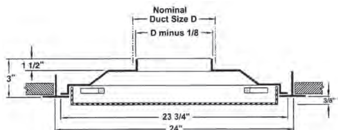
PDR3D (Drop Screen Lay-In)
