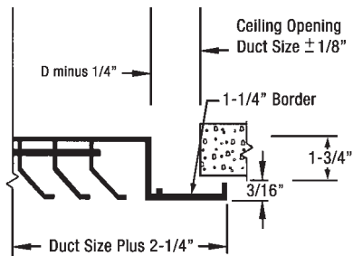
TM5 (Surface Mount, Flat Frame)
