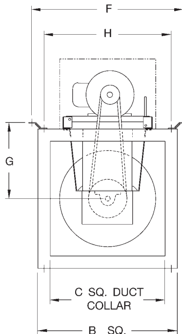
END VIEW
