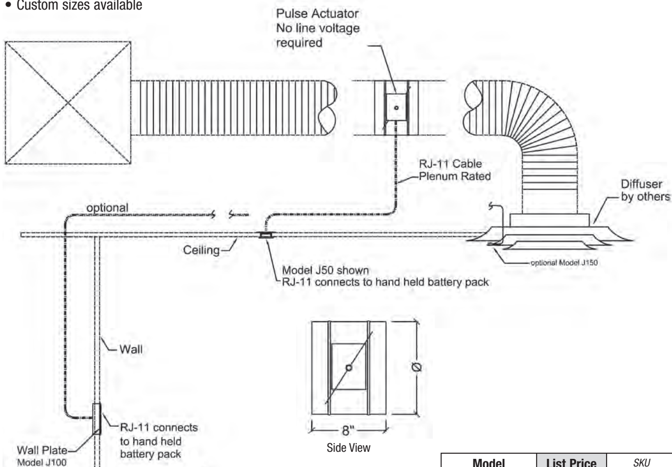
PB I3 shown above with optional hand held remote connected to a J50 terminal point.
