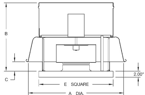
Models: DCRD60 through DCRD150
