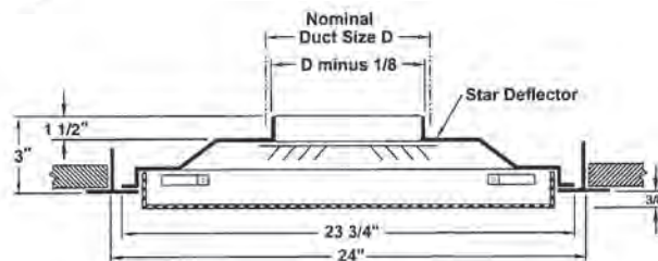
Model: PSS3D (Drop Screen Lay-In)
