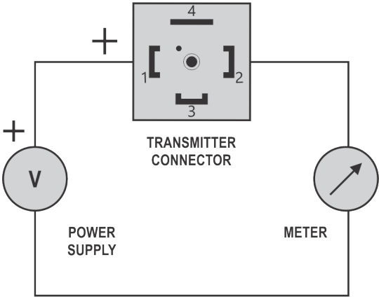
Figure 2 – Electrical connections
