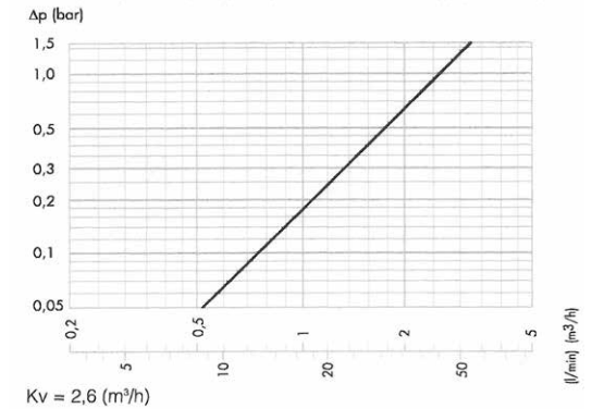
TV252140 / TV252150 FLOW RATE BY PRESSURE DROP
