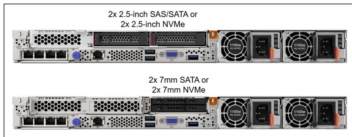
Figure 8. Rear drive bay configurations
