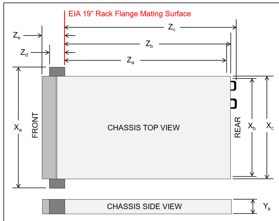
Figure 19. Server dimensions
