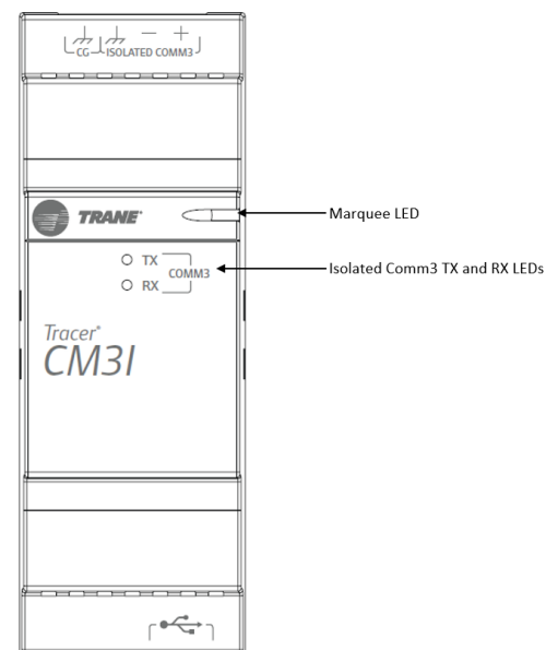
Figure 5. CM3I LEDs
