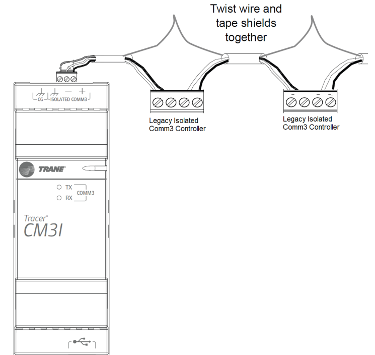
Figure 4. CM3I network wiring details
