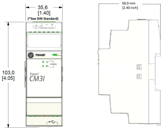
Figure 1. CM3I dimensions
