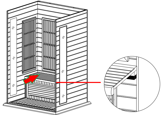
FIG-10 Installing Bench
