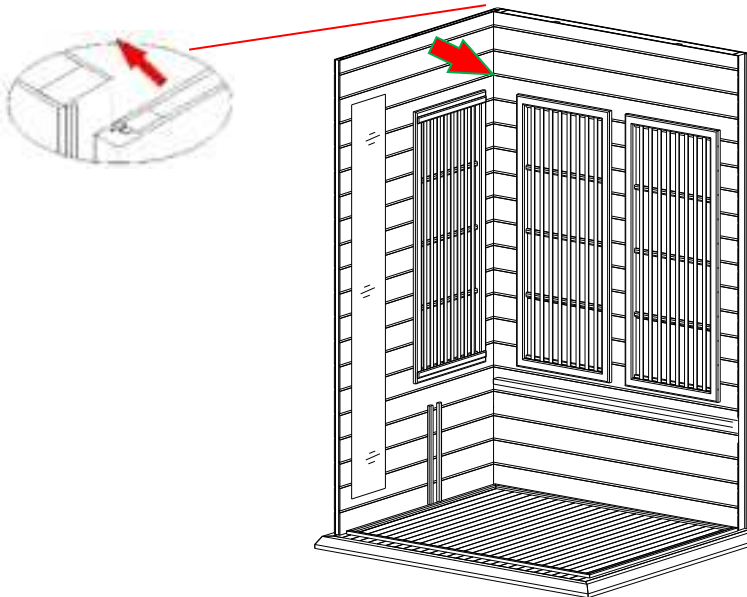
FIG-4 Assembling Left Side Panel
