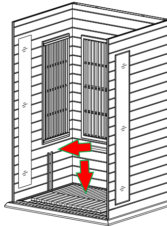
FIG-7 Placing Floor Heater
