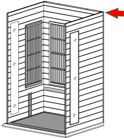
FIG-6 Assembling Right Panel
