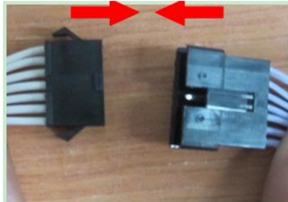
FIG-18 Connecting control panel connectors
