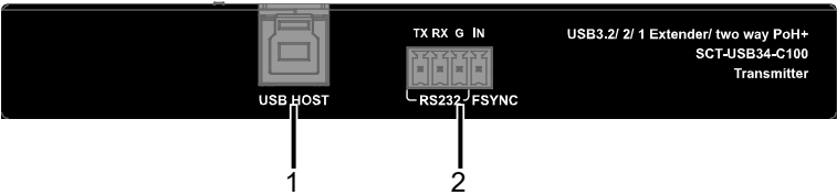
Front Panel
