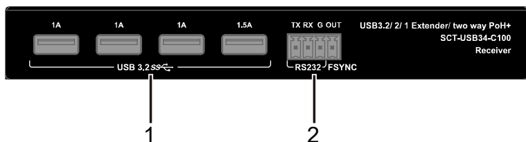
Front Panel
