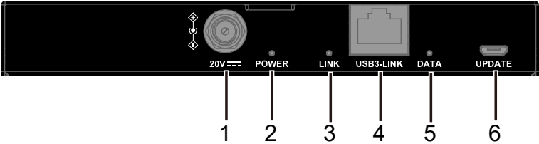
Rear Panel
