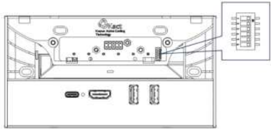
Figure 9: EXT3-C-WP-XR-T (EU/UK) DIP-Switches
