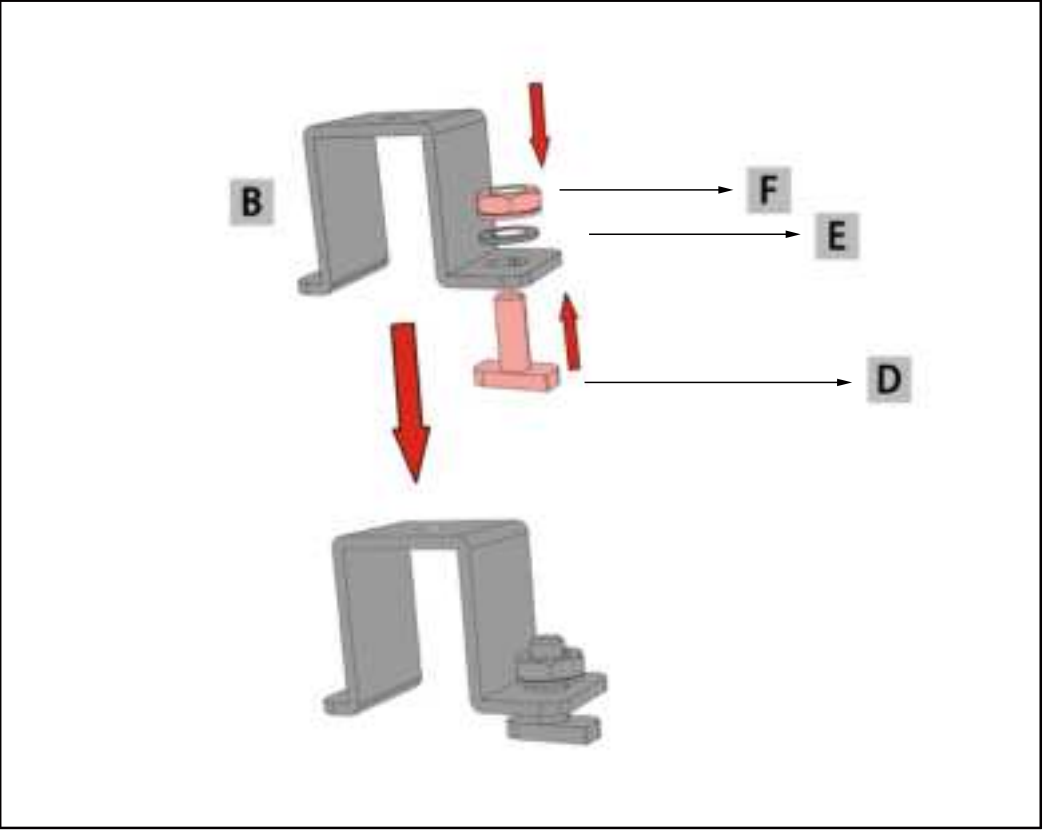
3. Install the accessories B,D,E,F as shown in the diagram. (Note: Do not tighten the screws).
