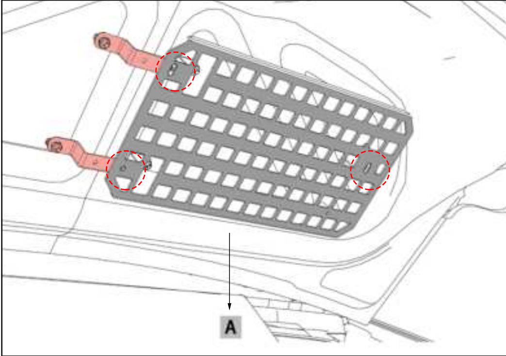
5.As shown in the diagram, align the molle panel on the right with the holes.
