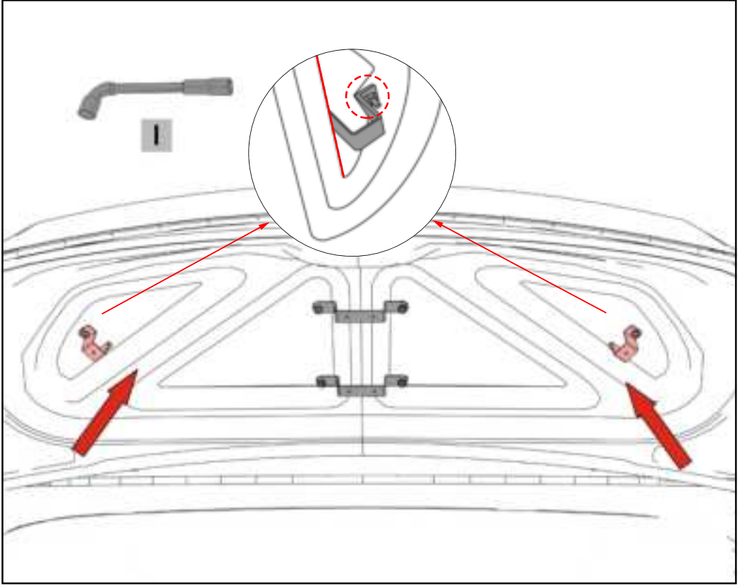
4. As shown in the diagram, fix the installed accessories to both sides inside the hood (insert one end of the accessory into the gap and the T-bolt into the round holes on both sides), adjust the position, and use tools to secure the nut.
