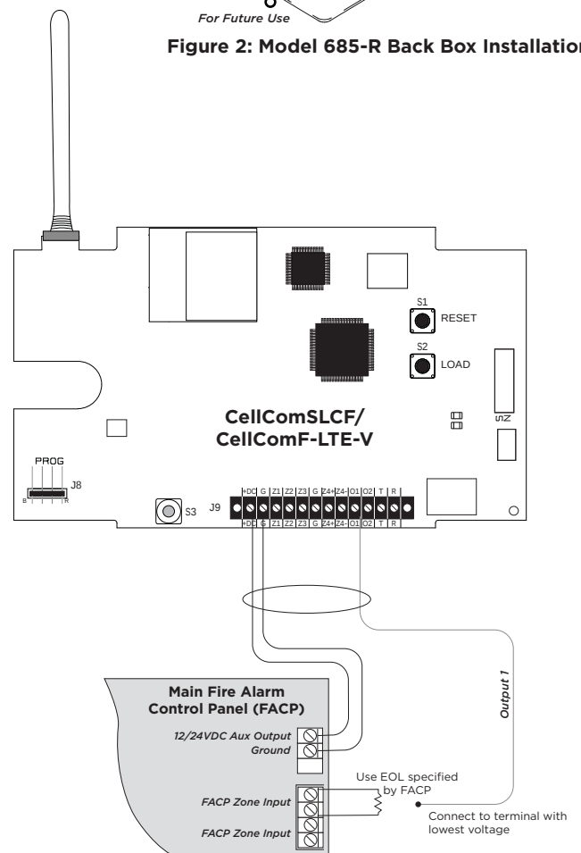
Figure 3: CellComSLCF and CellComF-LTE-V Wiring Diagram for FACP
