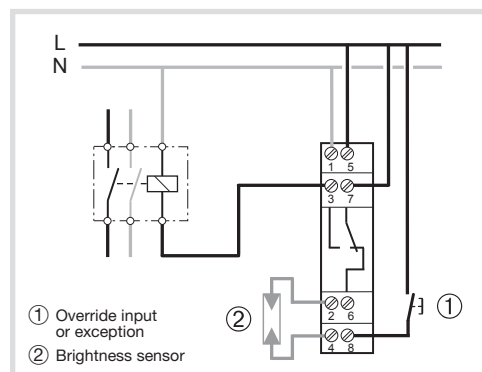
Figure 2: EGN100 connection diagram (1 output)
