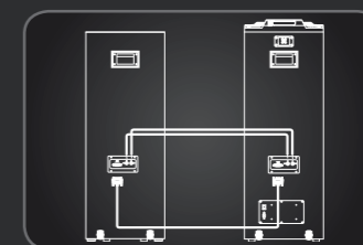
TWO SPEAKERS CONNECTION
