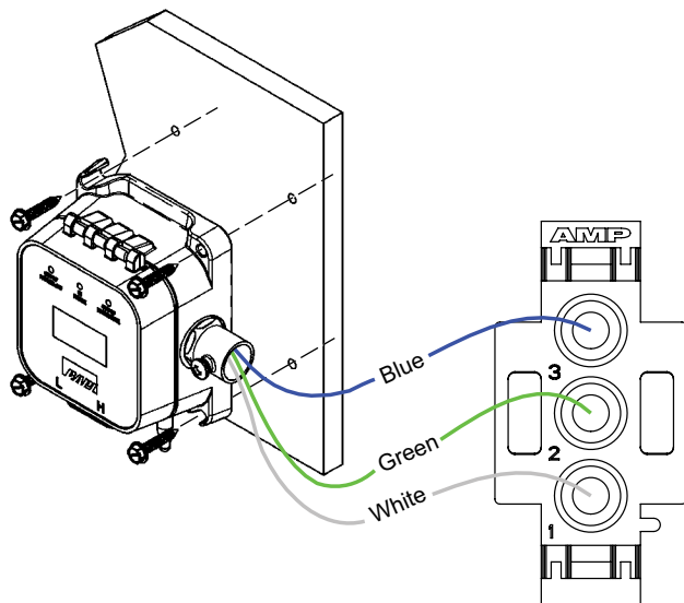
Figure 3: Sensor and Wiring Assembly
