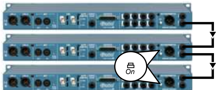
Linking multiple SW8-USB units using 1/4" TRS cables
