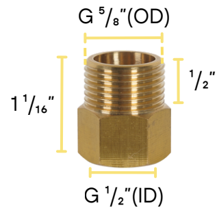
Brass Adapter
