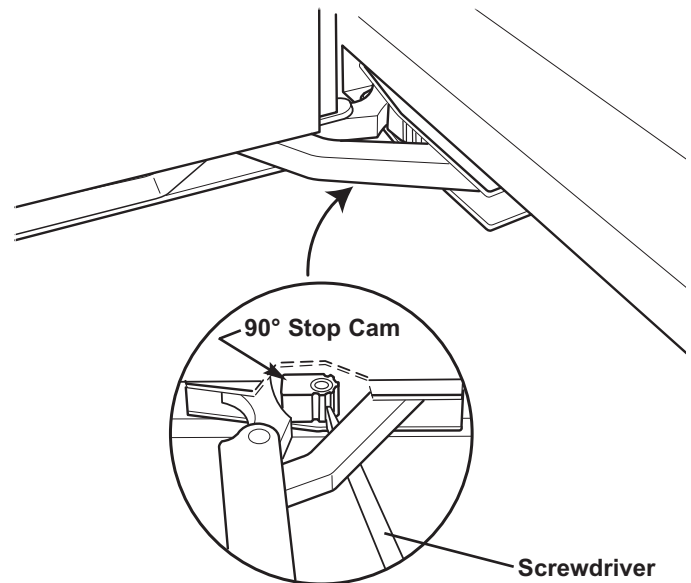
Figure 2-5. 90° Door Stop Cam
